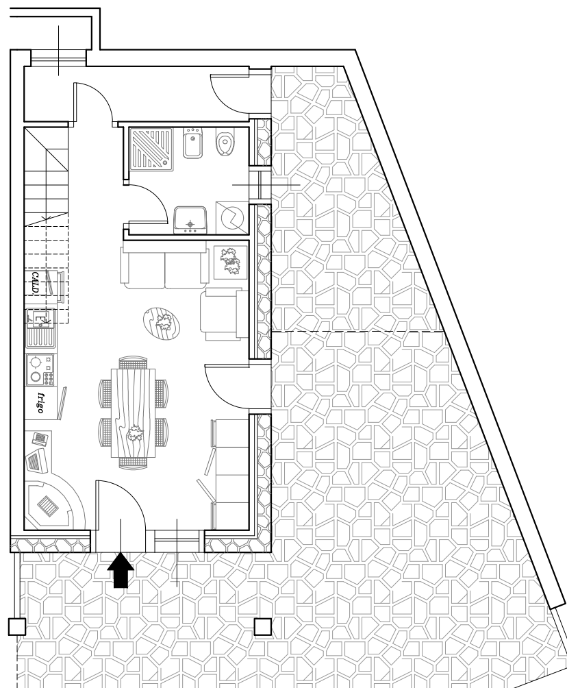
PIANO TERRA
